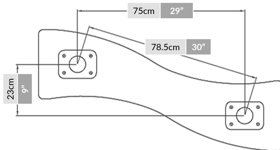
DUO SD Hole Centres
